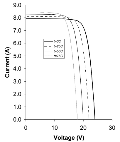
BP 3125 I-V Curves
